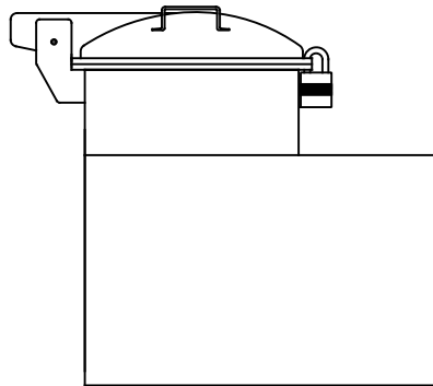
48" full tank penetration ring collar enclosure with offset locking hinged cover (and optional fiberglass ladder) (Download full tank penetration ring collar enclosure DWG here)
