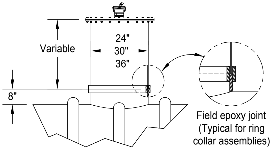
Bolted flat cover with ring collar tank joint and optional 4" locking inspection hatch ( Download bolted flat cover DWG here )
