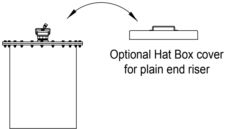
Bolted flat cover with ring collar tank joint and optional 4" locking inspection hatch ( Download bolted flat cover DWG here )
