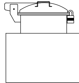
48" ring collar manway enclosure with locking hinged cover and internal bolted 20" manway (Download ring collar manway enclosure DWG here)
