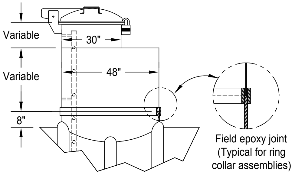
48" full tank penetration ring collar enclosure with offset locking hinged cover (and optional fiberglass ladder) (Download full tank penetration ring collar enclosure DWG here)
