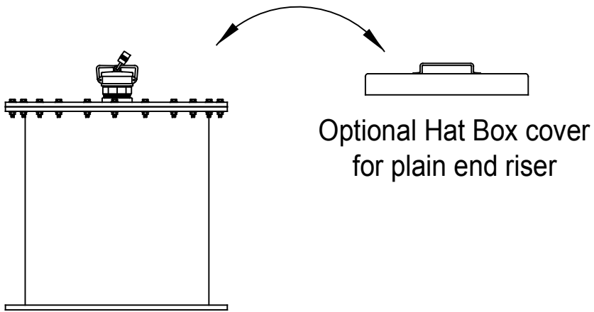
Bolted flat cover with bolted tank flange and optional 4" locking inspection hatch ( Download bolted flat cover DWG here )
