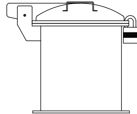
Locking hinged cover with bolted tank flange ( Download locking hinged cover DWG here )
