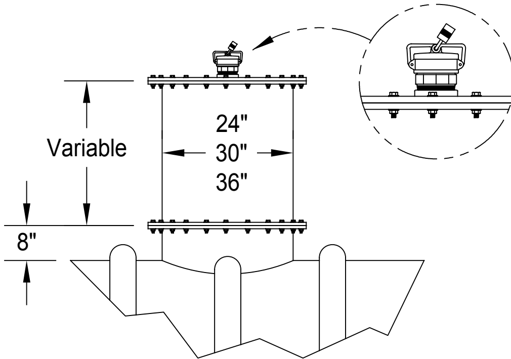
Bolted flat cover with bolted tank flange and optional 4" locking inspection hatch ( Download bolted flat cover DWG here )
