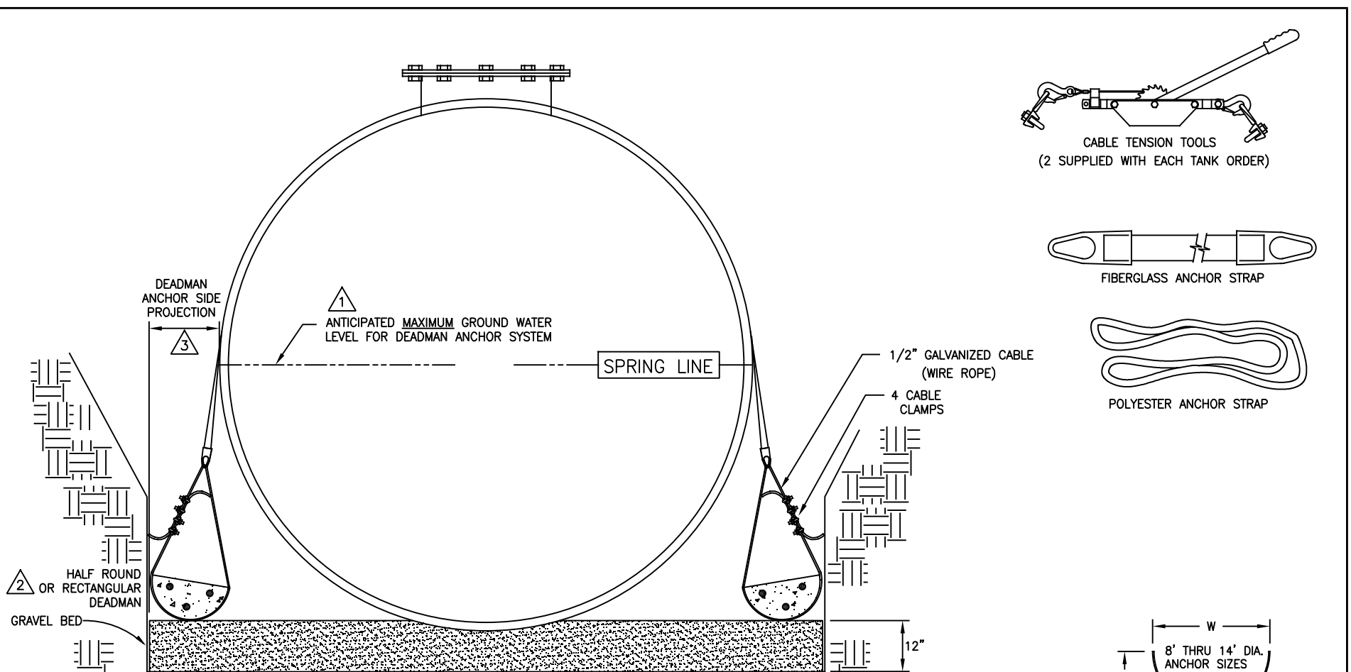
1 TRADITIONAL DESIGN DEADMAN ANCHOR DETAILS STANDARD CONDITIONS
