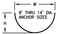
2 FIBERGLASS OR CARDBOARD DEADMAN FORM (USE HALF A CAISSON TUBE)
