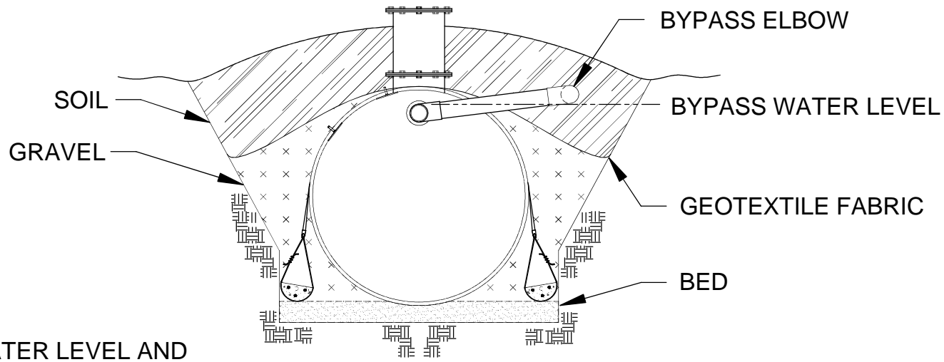
END VIEW
